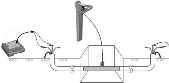
Fig.5.6 Sensor identification
