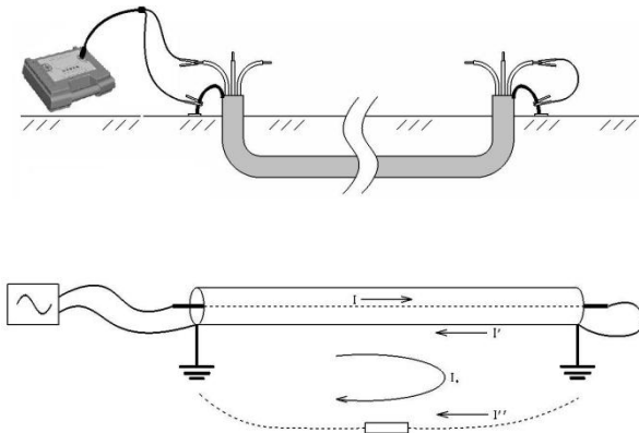
Fig.3.3 Phase-Sheath Method
