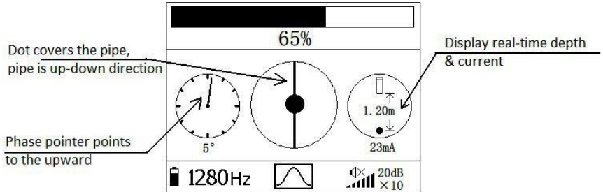
Fig.4.11 Real-time depth and current measurement
