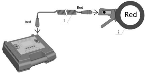
Fig.2.6 Clamp coupling accessories connection diagram
