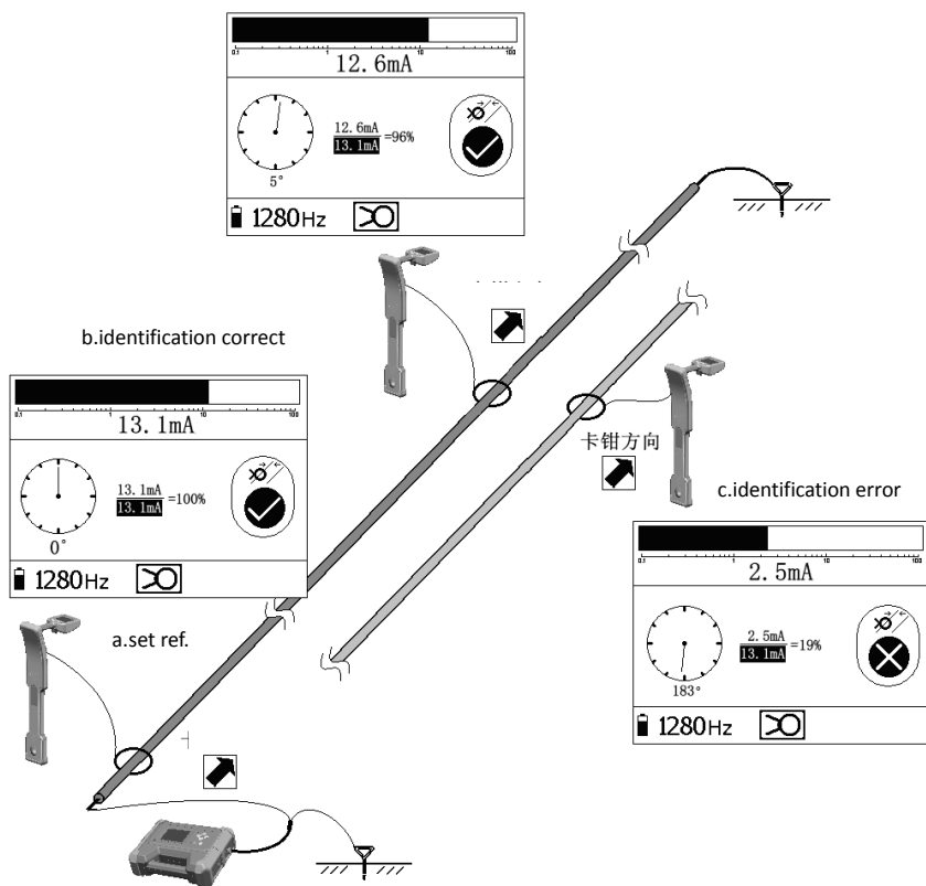
Fig.5.3 Clamp identification process
