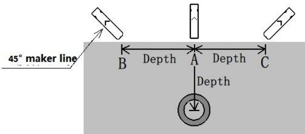
Fig.4.13 45% null manual depth measurement
