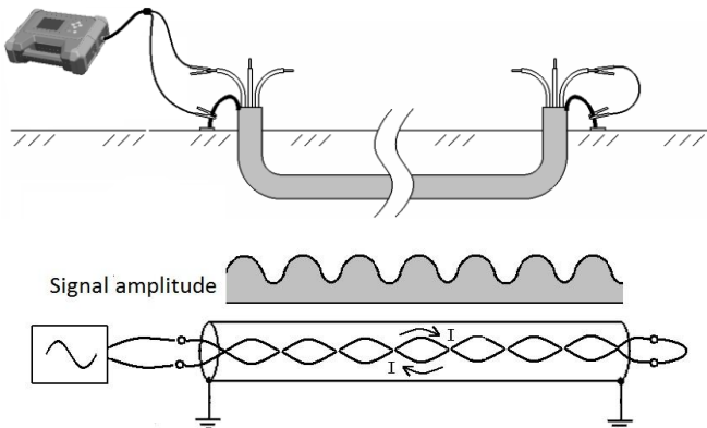
Fig.3.5 Phase-phase method
