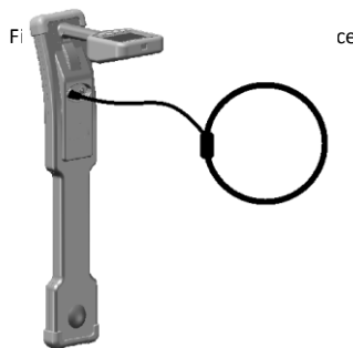
Fig.5.1 Receiver clamp connection
