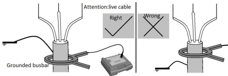
Fig.3..6 Clamp coupling method 1 (to clamp the cable)
