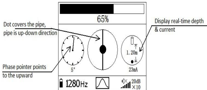
Fig.4.11 Real-time depth and current measurement
