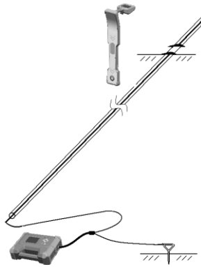
Fig.7.3 break fault testing wiring
