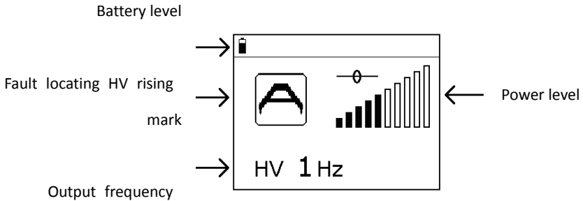
Fig.6.2 Transmitter fault locating HV rising output interface
