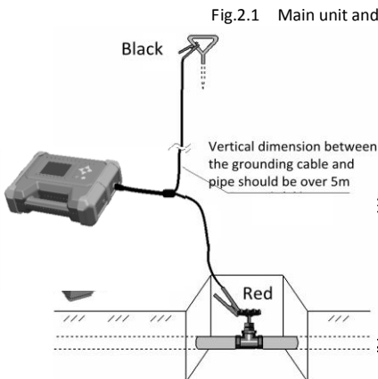
Fig.2.1 Main unit and accessories cable connection diagram
