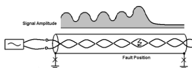
Fig.7.1 A frame fault locating process
