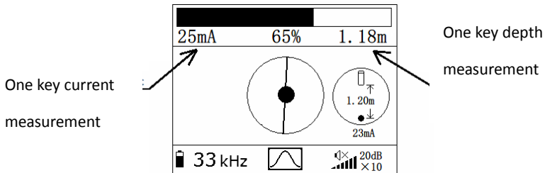
Fig.4.12 One-key depth and current measurement
