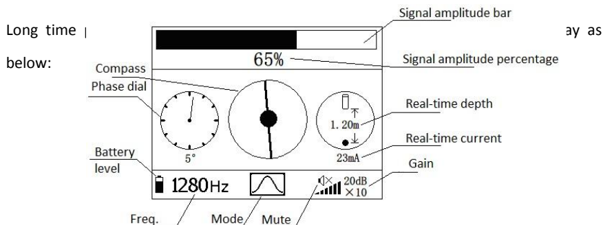
Fig.4.1 Pipe detection interface diagram
